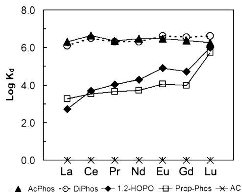
Fig. 3. Distribution coefficients ( K_d ) of lanthanides on various sorbents measured in 0.1 M \text{HCl}/\text{NaCl} (pH 2.42), initial [lanthanide] of \sim 50 ppb (each), L/S of 5000 mL/g.
