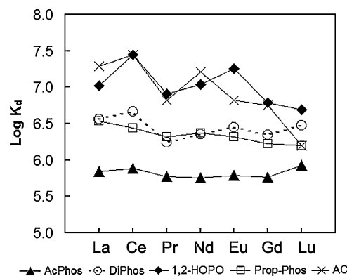
Fig. 5. Distribution coefficients ( K_d ) of lanthanides on various sorbents measured in ground water (pH 8.07), initial [lanthanide] of \sim 50 ppb (each), L/S of 5000 mL/g.
