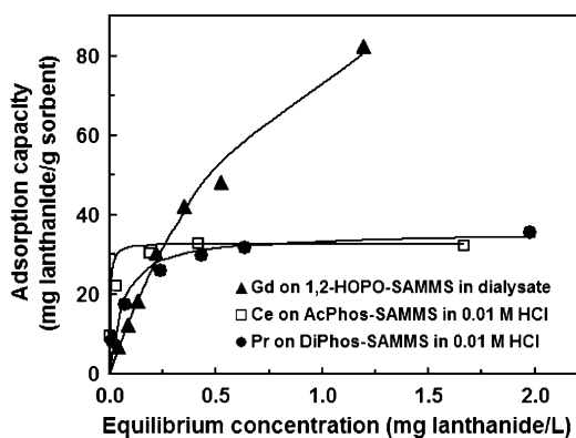
Fig. 9. Adsorption isotherms of Ce, Pr, and Gd on SAMMS materials measured in 0.01 M HCl for Ce and Pr and dialysate for Gd at L/S of 10^5 mL/g.
