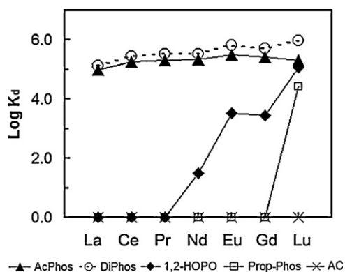
Fig. 2. Distribution coefficients ( K_d ) of lanthanides on various sorbents measured in 0.1 M \text{HNO}_3/\text{NaNO}_3 (pH 1.82), initial [lanthanide] of \sim 50 ppb (each), L/S of 5000 mL/g.
