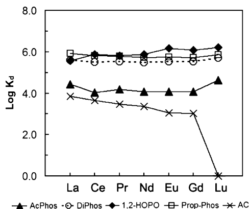
Fig. 7. Distribution coefficients ( K_d ) of lanthanides on various sorbents measured in dialysate (pH 8.33), initial [lanthanide] of \sim 50 ppb (each), L/S of 5000 mL/g.
