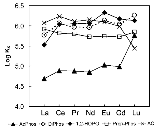
Fig. 6. Distribution coefficients ( K_d ) of lanthanides on various sorbents measured in sea water (pH 7.68), initial [lanthanide] of \sim 50 ppb (each), L/S of 5000 mL/g.
