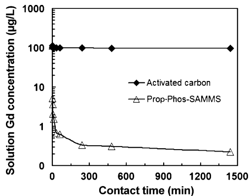
Fig. 8. Adsorption kinetics of Gd on SAMMS and activated carbon in dialysate (pH 8.33), initial [Gd] of \sim 100 ppb, L/S of \sim 5000 mL/g.
