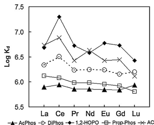
Fig. 4. Distribution coefficients ( K_d ) of lanthanides on various sorbents measured in river water (pH 7.98), initial [lanthanide] of \sim 50 ppb (each), L/S of 5000 mL/g.
